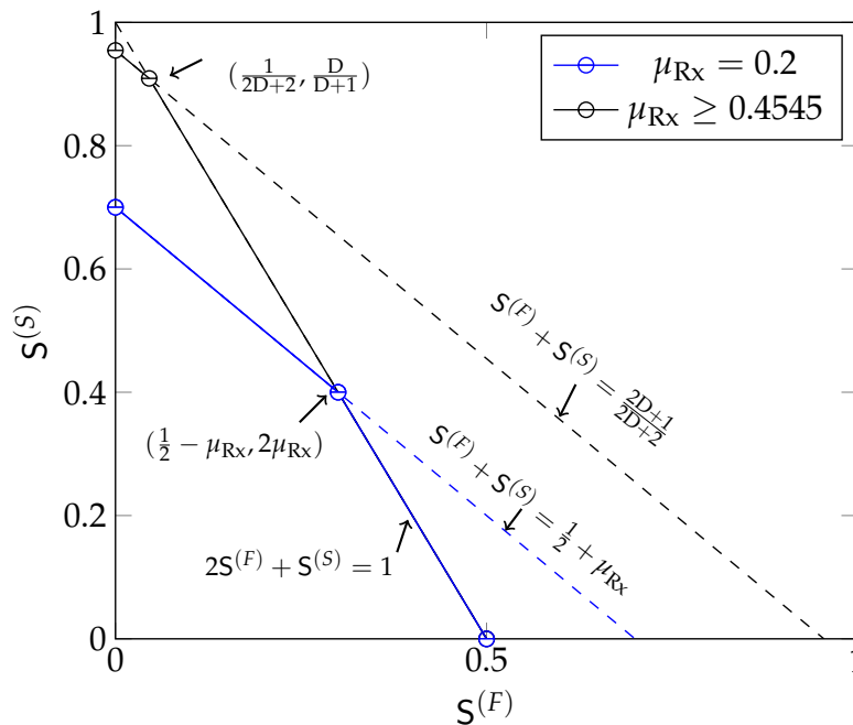
Figure 2. The optimal MG region \mathcal{S}_{Rx}^*(\mu_{Rx}, D) for Rx-cooperation only, for different values of \mu_{Rx} and D = 10 and L = 1 .
