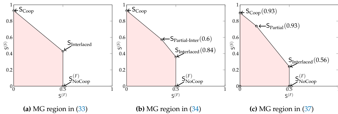
Figure 6. Examples of the three MG regions in (33), (34) and (37). Specifically, we used D_{Tx} = 3, D_{Rx} = 3 , and \mu_{Tx} \in \{0.4, 0.3, 0.2\} and \mu_{Rx} \in \{0.4, 0.3, 0.2\} .
