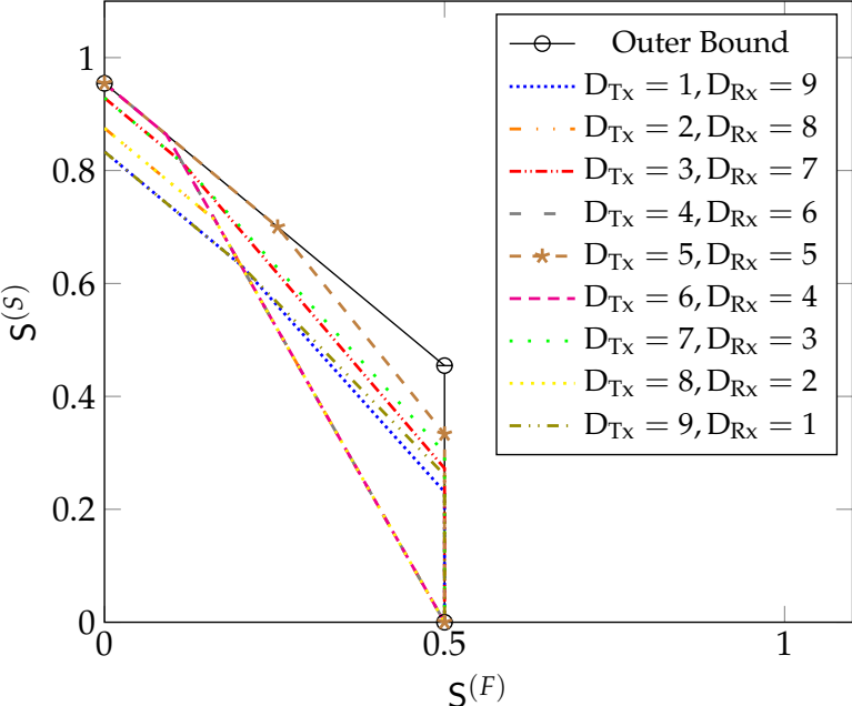
Figure 9. Bounds on S^*(\mu_{Tx}, \mu_{Rx}, D) for \mu_{Tx} = 0.3, \mu_{Rx} = 0.3, D = 10 and L = 1 with both Tx- and Rx-cooperation.
