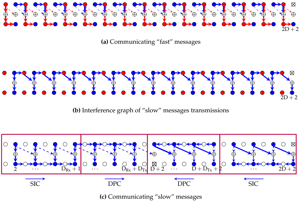
Figure 12. An illustration of the scheme achieving MG pair (31e). Notice that since D is even, the last Tx of \mathcal{G}_2 sends a "fast" message. And since D_{Rx} is odd, also the first Tx in \mathcal{G}_4 sends a "fast" message.
