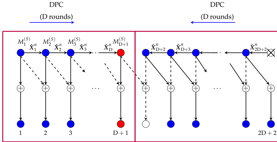
Figure 5. Scheme for Tx-cooperation only.
