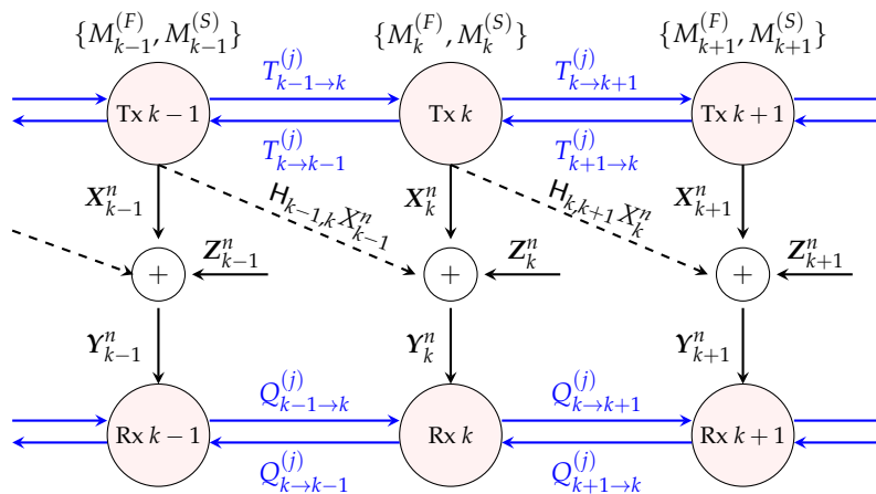
Figure 1. System model with transmitter (Tx-) and receiver (Rx-) cooperation.
