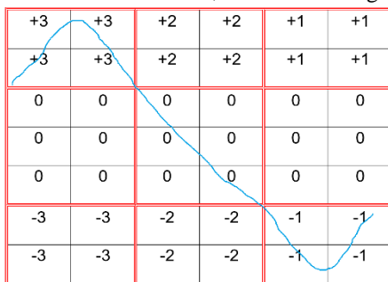
Convolution value = +5
