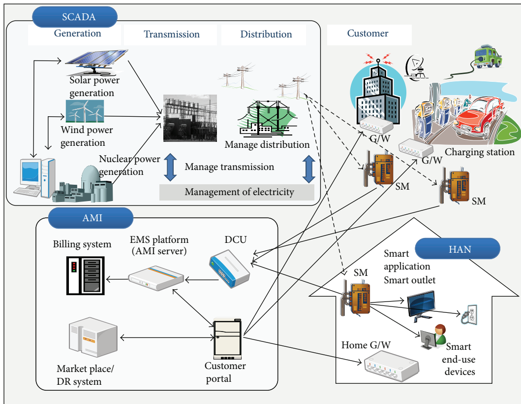
FIGURE 1: Communication structure of smart grid.
