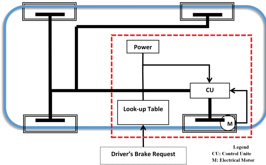
Figure 1. Proposed BBW architecture for one-wheel brake model.
