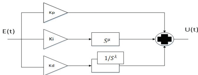
Figure 9. Fractional-order PID controller.
