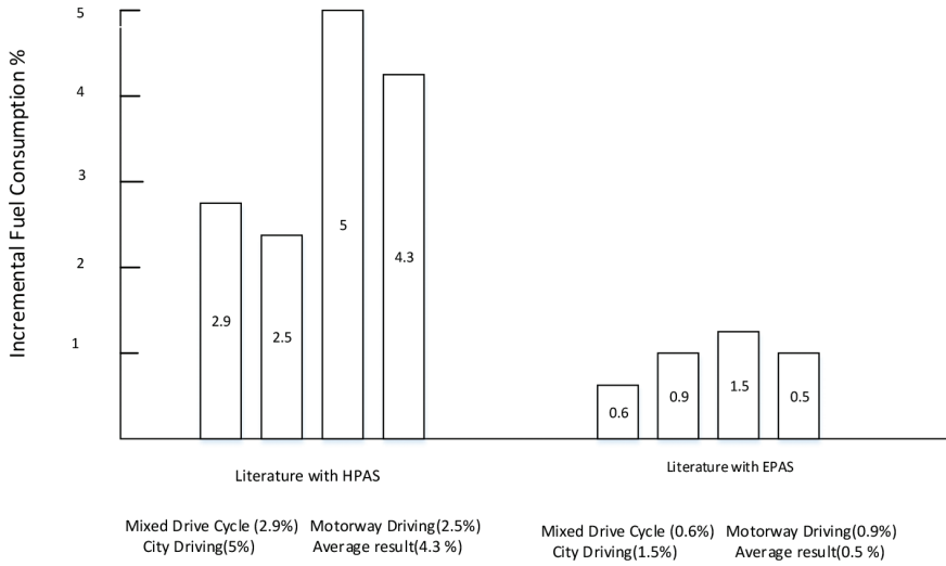
Figure 7. Typical EPAS fuel consumption saving.
