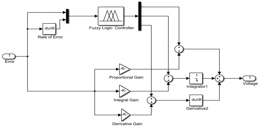
Figure 4. Fuzzy-PID controller (MATLAB Simulink scheme).
