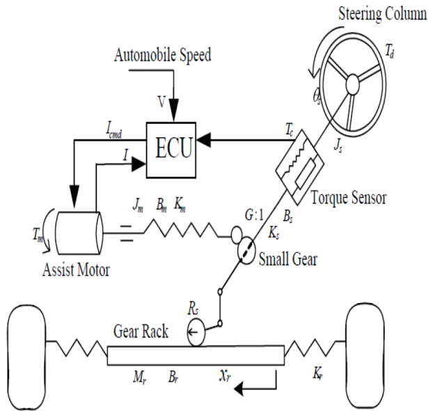
Figure 8. EAPS dynamic model.
