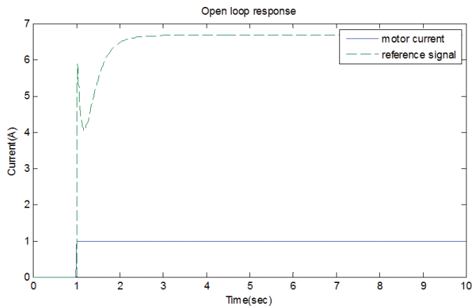
Figure 12. Unit step response of EPAS open-loop system.
