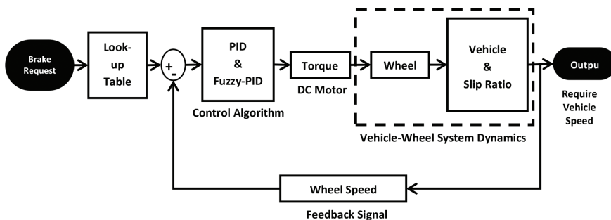
Figure 3. BBW control system design.
