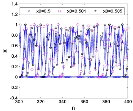
Fig. 5 The sensitivity of initial condition in chaotic system.
