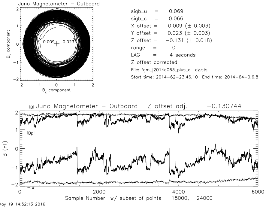
Fig. 44 Application of offset estimation to range 0 ( \pm 1600 nT dynamic range) observations obtained during cruise. The figure in the upper left is a diagnostic hologram of B_y vs. B_x . In the lower figure a time series of the field magnitude and the negative of the field magnitude is shown ( dotted lines ) demonstrating little spin modulation of the magnetic field magnitude with the estimated offsets applied to the observations. The spin axis component of the field ( z axis) and the spin plane component ( \rho ) are shown, illustrating a few Alfvénic (magnitude-preserving) fluctuations in the solar wind that may be used to estimate offsets in z
