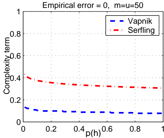
Figure 3: The complexity term of the Vapnik and Serfling bounds as a function of p(h) with 0.01 \leq p(h) \leq 1 , \delta = 0.01 and m = u = 50 .
