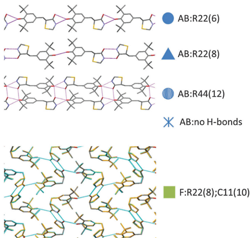
Fig. 4. The crystal energy landscape for racemic tazofelone, with the key to the hydrogen bonding motifs. The figure for F:R22(8);C11(10) is an overlay of this sheet in the three racemic polymorphs, adapted from ref. 19.
