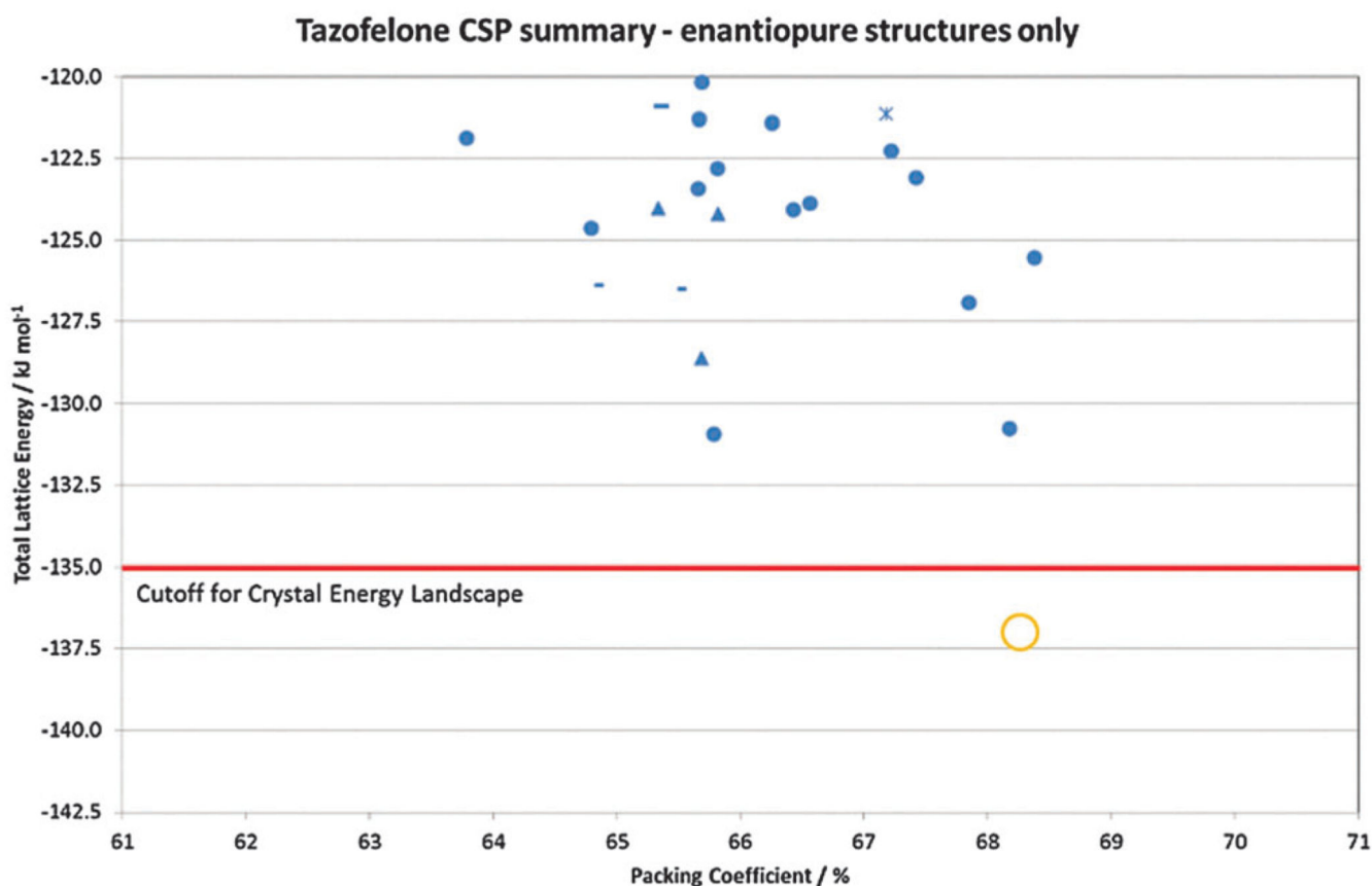
Fig. 5. Summary of the CSP generated enantiopure structures for tazofelone adapted from ref. 19. The experimental structure is Z' = 2 and hence not found in the Z' = 1 search ( Z' is the number of independent molecular conformations in the crystal.) The horizontal line is the cutoff used for the crystal energy landscape (Fig. 4) that was applied to the CSP summary (Fig. 3) for crystal structures that could be obtained from a racemic mixture.
