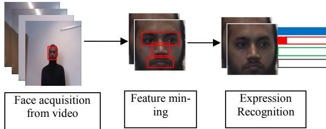
Figure 11-3 Steps of a typical facial expression recognition system.
