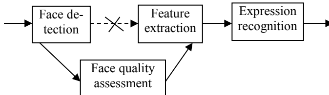
Figure 11-5 Face quality is assessed before feature extraction is attempted for expression recognition.
