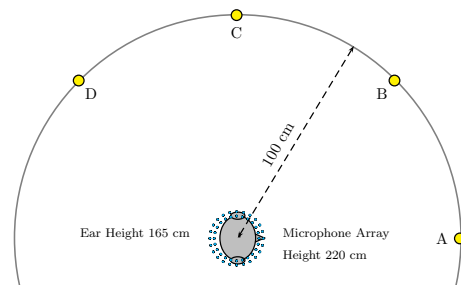
Fig. 3. Setup for real-room speech recordings. The 48-channel microphone array was hung right above the dummy head, to record concurrent speech signals coming from position pairs (A,B), (A,C) and (A,D).
