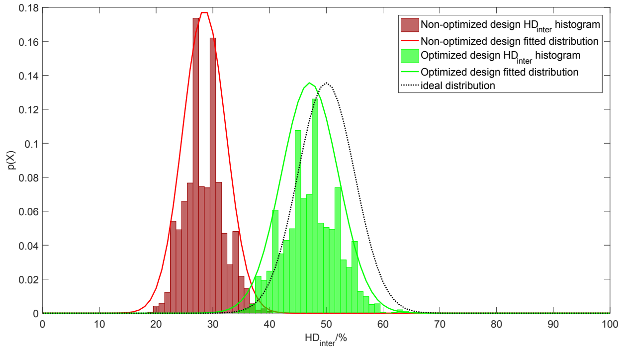
Figure 6. TERO-PUF uniqueness
