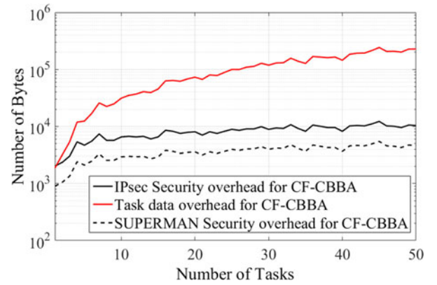
Fig. 10. Chart to compare the number of additional bytes required for the security overhead of IPsec and SUPERMAN when performing CF-CBBA.
