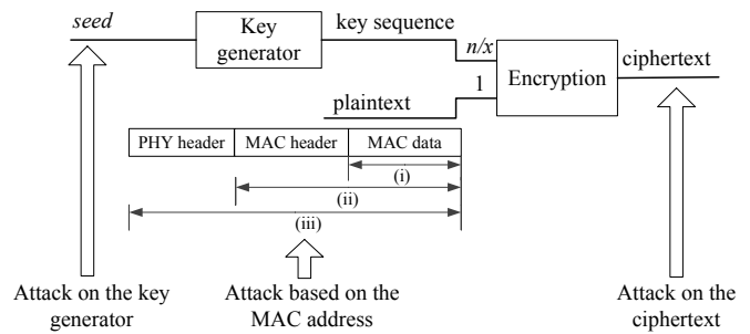
Fig. 1. Encryption schemes and security attacks. (i), (ii), and (iii) are different fields protected by MAC layer encryption schemes, most PLE schemes and our PLE scheme, respectively; n and x is key-to-data ratio for other PLE schemes and our scheme, respectively. The security analysis of these three attacks is presented in Section IV.
