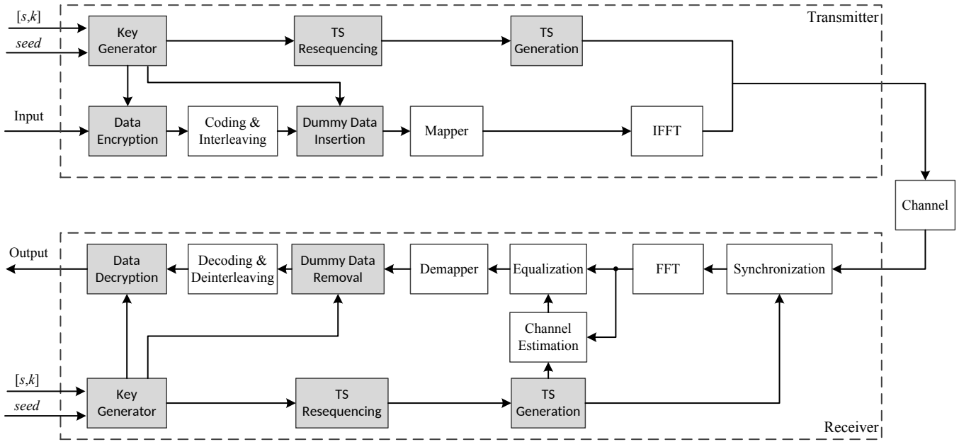
Fig. 4. The block diagram of the proposed OFDM PLE system. The gray blocks are added for encryption and decryption.
