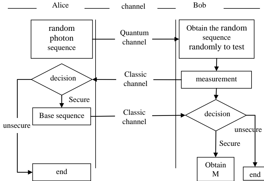
Figure 1. The Proposed Unidirectional Transmission Protocol
