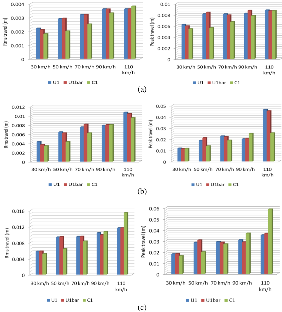
Fig. 16: Comparisons of the rear-right suspension travel with different suspension configurations under different road conditions: (a) responses under smooth road inputs; (b) responses under medium-rough road inputs; (c) responses under rough road inputs.
