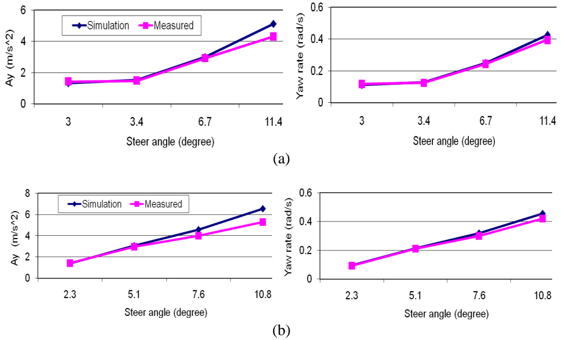
Fig. 6: Comparisons of lateral acceleration ( A_y ) and yaw rate responses of the vehicle model with the measured data reported in [22] under a steady-state turning maneuver: (a) forward speed = 12 m/s; (b) forward speed = 14.3 m/s.
