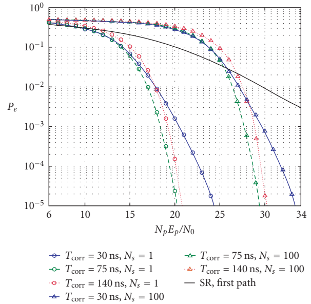
FIGURE 12: Comparison of TR- and SR-UWB systems. Note that N_p E_p / N_0 = E_b / N_0 is the bit-energy-to-noise-power density ratio, and N_s = N_p / 2 is the number of pulse pairs used to represent a bit.
