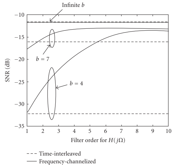
FIGURE 9: SNR versus lowpass filter order.
