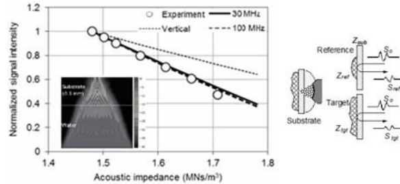
Figure 1. Signal intensity as a function of acoustic impedance of the target. Normalized by the intensity when water is the target. Substrate: polystyrene. Vertical: assuming vertical incidence.
