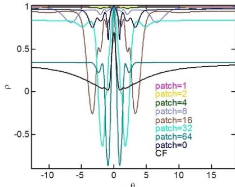
Fig. 2: Plots of Odd/Even Aperture Coherence (OEAC) coefficient of a dot in homogeneous speckle environment for different patch size. Black line is coherence factor (CF) for comparison.
