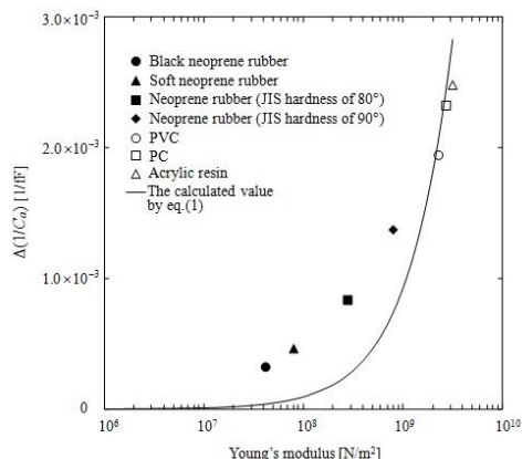
Fig.1 Measured \Delta(1/C_a) vs Young's moduli of materials for neoprene rubbers and plastics. The solid line is the calculated value of \Delta(1/C_a) .
