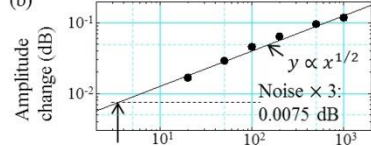
Detection limit: 3.7 ppm H 2 concentration (ppm) Fig.2 Measurement of H 2 gas (a) Amplitude response (b) concentration dependence of response
