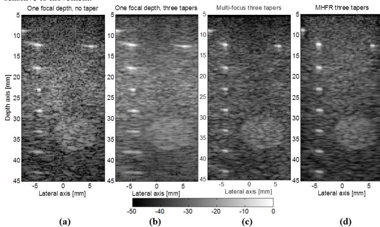
Figure : Log compressed (dB) images of cyst and wires from the UlaOp scanner, (a - b) one focal depth at 22.5 mm without and with three tapers apodization in reception, (c) MF with three tapers apodization in reception and (d) MHFR with three tapers apodization in reception and 61 transmitted angles.
