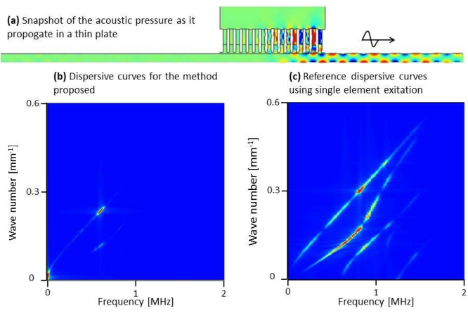
Figure 1: (a) A snapshot of the propagated wave at time t = 30\text{ms} (b) Dispersive curves calculated by FFT in time and space of the plate's surface displacements; the dominance of A_0 mode can be clearly seen, and (c) Reference dispersive curves for the same setup, but with a single element excitation; wave propagation with A_0 together with S_0 , A_1 , S_1 , S_2 can be seen.
