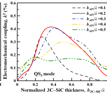
Figure 1(b). Simulated electromechanical coupling dispersion of the QS_3 mode in an AIN/3C-SiC layer.
