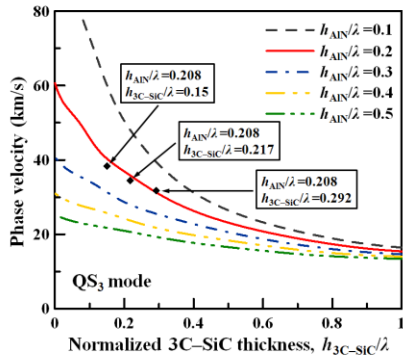
Figure 1(a). Simulated phase velocity dispersion of the QS_3 mode in an AIN/3C-SiC layer.
