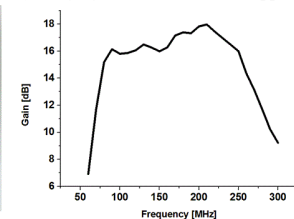
Fig. 1. (a) Designed power amplifier (left, Dimension : 96.52x63.5 mm 2 ) and (b) measured gain(right)
