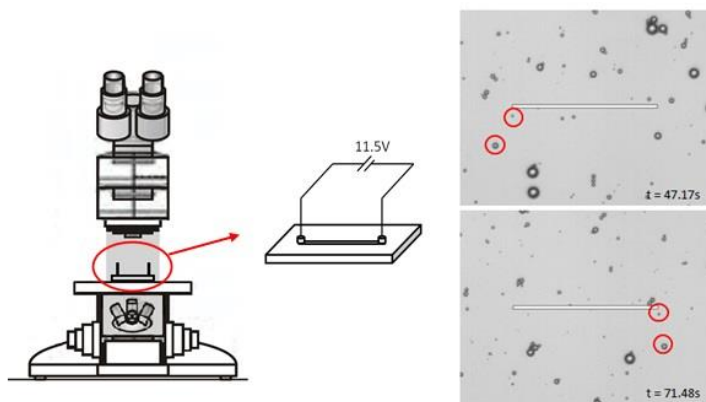
Figure 1 - Schematic representation of experimental setup. MB suspension was flowed into an ibidi™ microchannel (channel dimensions: L=5\text{cm} , w=0.5\text{cm} , h=200\mu\text{m} ) and a potential of 11.5V was applied. MB movement over time was then recorded to determine MB surface charge. Right: Images of SonoVue™ MBs movement in an applied over time (Scale bar represents 100\mu\text{m} ).
