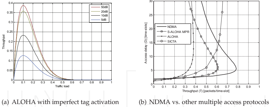
Fig. 3. Performance of MAC algorithms with cross-layer optimization
