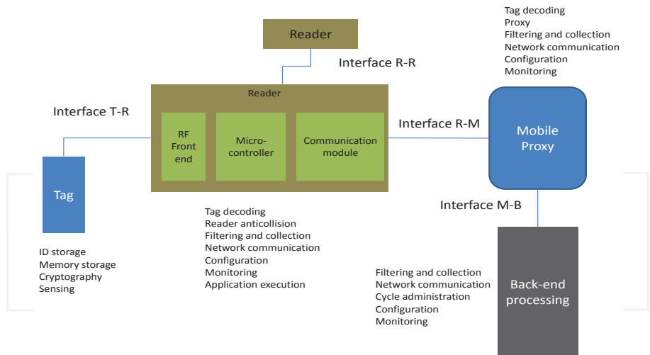
Fig. 1. Reference RFID system architecture
