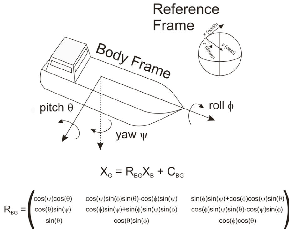
Figure 9. Compensation for pitch, roll and yaw of the camera platform. The body frame is attached to a ship or platform and reference frame attached to Earth. By knowing the position C_{BG} of the body in the world and the yaw, pitch and roll angles, a point X_B in the bodies local coordinate system can be transformed into a point X_G in the global reference frame. The X-axis is positive towards the bow/front of the vessel/vehicle, the Y-axis is positive towards starboard and the Z-axis is positive downward. Consequently, the roll angle around the X-axis is positive when the port-side of the vessel/vehicle come up; pitch angles around the Y-axis are positive when the bow comes up; yaw/heading angles around the Z-axis are positive clockwise.
