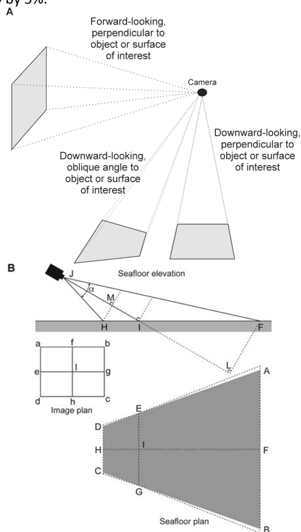
Figure 6. Camera orientations to the object, area or volume of interest, and the resulting image shapes (A). Dimensions used in the calculation of dimensions in a perspective grid (B), after Wakefield & Genin (1987). Image corners are identified A-D, with mid-points added as E-I. Corresponding seafloor locations are identified as A-I. Location J is the camera focal point and the vertical acceptance angle ( 35^\circ ) is indicated as \alpha (the horizontal acceptance angle, \beta , of 45^\circ is not illustrated). Locations L and M fall on the central axis of the camera such that JL and JM represent the appropriate object distances for seafloor points on lines AB and CD, respectively. The resultant seafloor area imaged is the shaded area ABCD, the same area estimated by the Wakefield & Genin (1987) methodology is shown as the corresponding dashed line. Note that they use distance JF rather than JL to represent the distance to the camera of objects along CD, and likewise use JH rather than JM as the distance of objects along AB. In this example, the latter method overestimates lengths DC and AB, and area ABCD by 5%.
