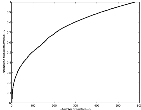
Figure 4: \frac{I(\tilde{X}, Y)}{I(X, Y)} Vs Number of clusters.
