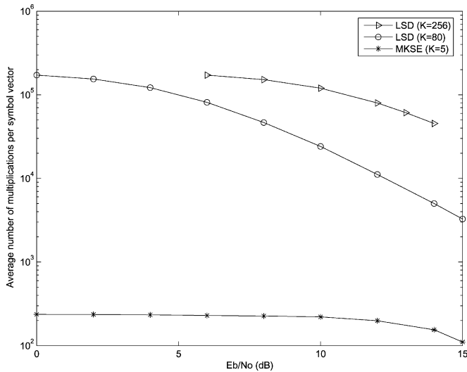
Fig. 10. Complexity comparison between MKSE and LSD, 4 \times 4 16-QAM.
