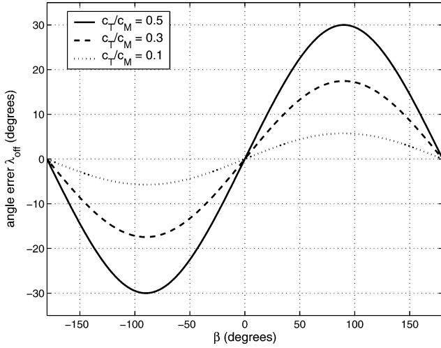
Fig. 6 Errors induced by using information patter \mathcal{I}_2 . Angle error \lambda_{\text{off}} vs desire approach angle \beta for three values of c_T/c_M , the ratio of target speed to missile speed.
