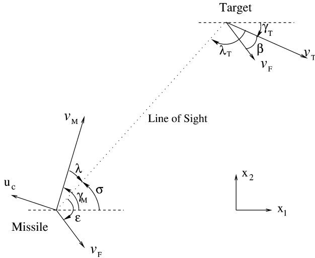
Fig. 1 Engagement geometry.
