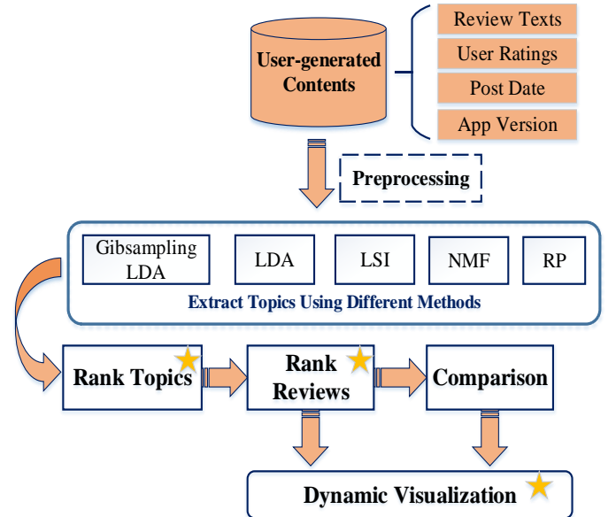
Fig. 1: Framework of AR-Tracker
