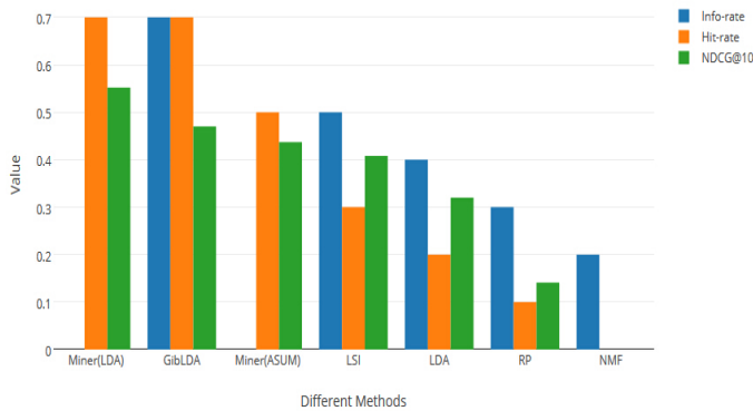
Fig. 4: Comparison of Different Methods
