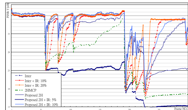
Fig. 6. Frame by frame PSNR comparison of Inter-MCP, 2HMCP, and proposed 2HMCP with three IR rates for Foreman (PLR = 5%, QP = 24, pattern #7)
