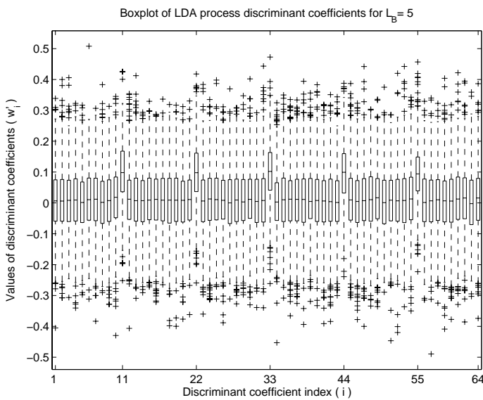
Fig. 5. Boxplot of 1000 discriminant coefficient sets of LDA trained by 1000 impostor (class I ) and 6 client (class C_3 ) vectors. The ‘most discriminant’ coefficients are indexed at 11, 22, 33, 44 and 55 on the x -axis.
