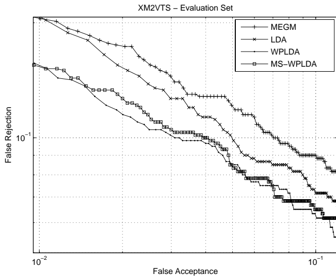
Fig. 8. ROC curve of XM2VTS – evaluation set experiments that are carried out under the and Lausanne protocol. The relevant training procedure for LDA, WPLDA, and MS-WPLDA uses 6 client similarity vectors and 1791 impostor similarity vectors. MEGM indicates the classification performance before training.
