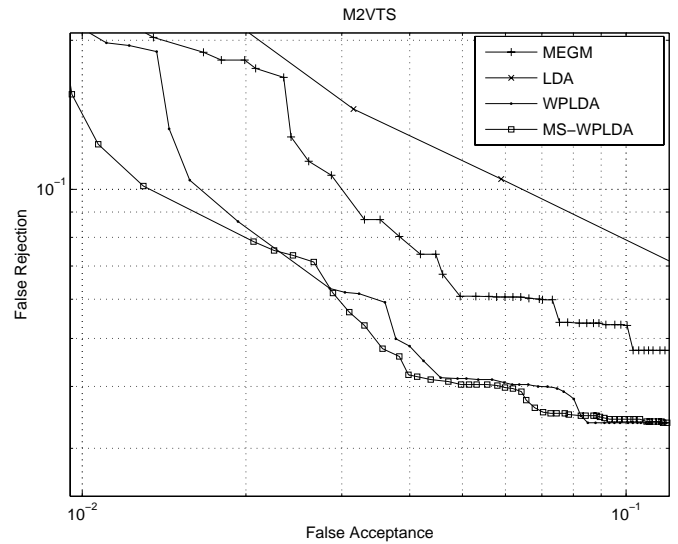
Fig. 7. ROC curve of M2VTS experiments that are carried out under the Brussels protocol. The relevant training procedure for LDA, WPLDA, and MS-WPLDA uses 6 client similarity vectors and 210 impostor similarity vectors. MEGM indicates the classification performance before training.
