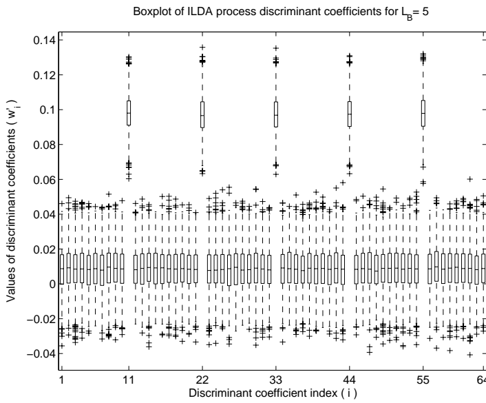
Fig. 4. Boxplot of 1000 discriminant coefficient sets of ILDA trained by 1000 impostor (class I ) and 6 client (class C_3 ) vectors. The ‘most discriminant’ coefficients are indexed at 11, 22, 33, 44 and 55 on the x -axis.
