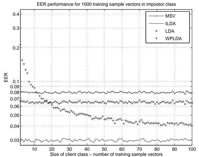
Fig. 3. EER when varying the number of client sample vectors selected from class C_3 and for 1000 impostor training vectors selected from class I . These sample vectors are used to train LDA and WPLDA whereas ILDA indicates the ideal performance and MSV the performance before training is used.
