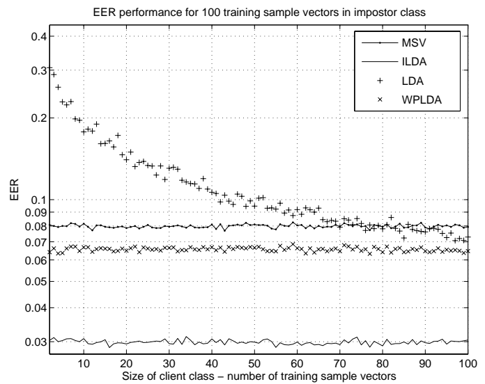
Fig. 2. EER when varying the number of client sample vectors selected from class C_3 and for 100 impostor training vectors selected from class I . These sample vectors are used to train LDA and WPLDA whereas ILDA indicates the ideal performance and MSV the performance before training is used.
