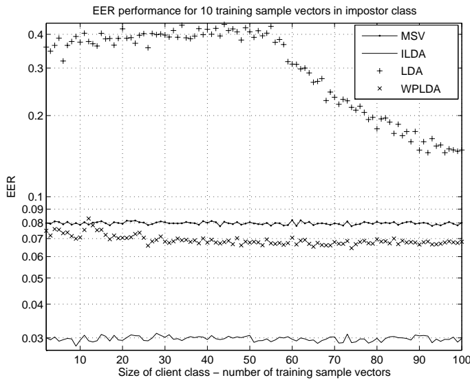
Fig. 1. EER when varying the number of client sample vectors selected from class C_3 and for 10 impostor training vectors selected from class I . These sample vectors are used to train LDA and WPLDA whereas ILDA indicates the ideal performance and MSV the performance before training is used.
