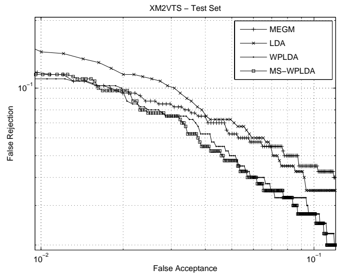
Fig. 9. ROC curve of XM2VTS – test set experiments that are carried out under the and Lausanne protocol. The relevant training procedure for LDA, WPLDA, and MS-WPLDA uses 6 client similarity vectors and 1791 impostor similarity vectors. MEGM indicates the classification performance before training.
