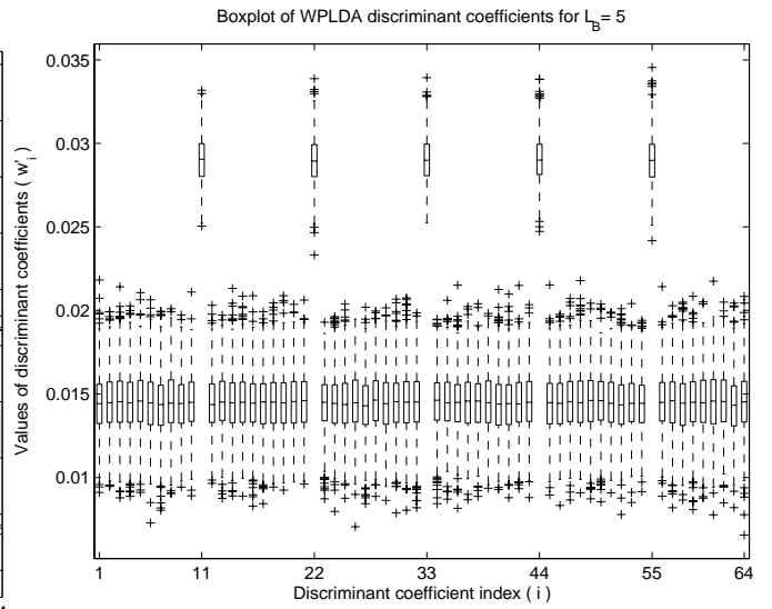
Fig. 6. Boxplot of 1000 discriminant coefficient sets of WPLDA trained by 1000 impostor (class I ) and 6 client (class C_3 ) vectors. The ‘most discriminant’ coefficients are indexed at 11, 22, 33, 44 and 55 on the x -axis.
