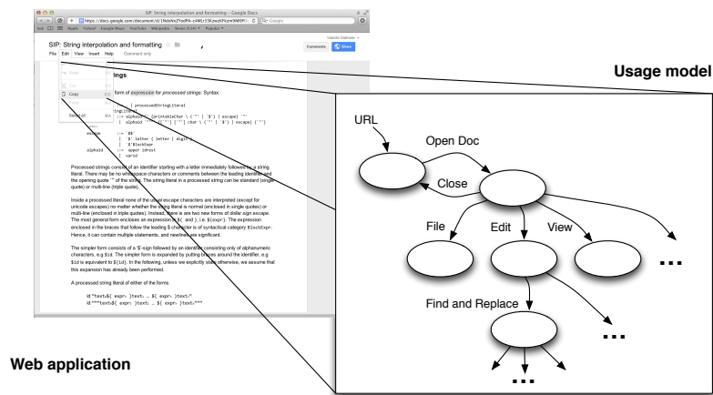
Figure 2: Simplified example of a usage model. States in the model correspond to different states of the application, whereas transitions in the model occur due to user interactions.
