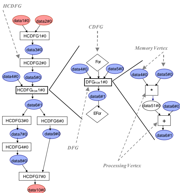
Figure 3 : HCDFG structure
