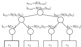
Figure 1: Example of a Merkle hash tree.
