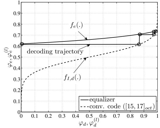
Fig. 1. Equalizer and decoder correlation characteristics for a random channel realization ( L = 32 , \tau_d = 5 ) at E_b/N_0 = 3 dB.
