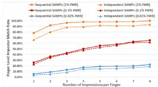
Fig. 8: Finger-level Imposter Match Rate variation as a function of the number of impressions per finger using the top 5 partial fingerprint based SAMPs from the FVC 2002 DB1-A dataset. Just as in the case of the capacitive dataset, here too, the sequential SAMPs performed better than the independent SAMPs. Further, the partial fingerprint based SAMPs performed much better than that of the full fingerprint based SAMPs (see Figure 6).
