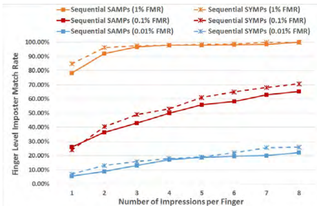
Fig. 13: Finger-level Imposter Match Rate using the partial fingerprint based SAMPs and SYMPs on the FVC 2002 DB1-A dataset. The IMR of SYMPs is observed to be better than that of SAMPs by \approx 3\% . Overall, the partial fingerprint based SYMPs continued to perform better than the full fingerprint based SYMPs shown in Figure 11.
