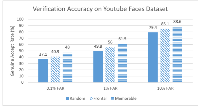
Figure 8. Comparing the performance of the proposed algorithm with random, frontal and memorable frames at different FARs.
