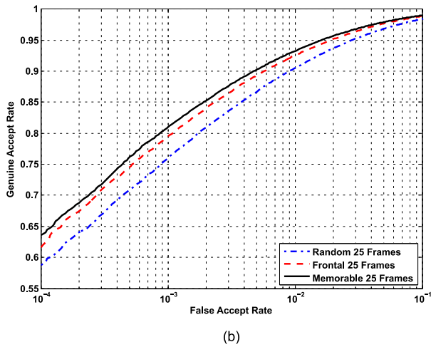
Figure 4. Evaluating the effectiveness of memorable frames by comparing with randomly selected frames and frontal frames on the (a) handheld and (b) control video sets of the PaSC database.
