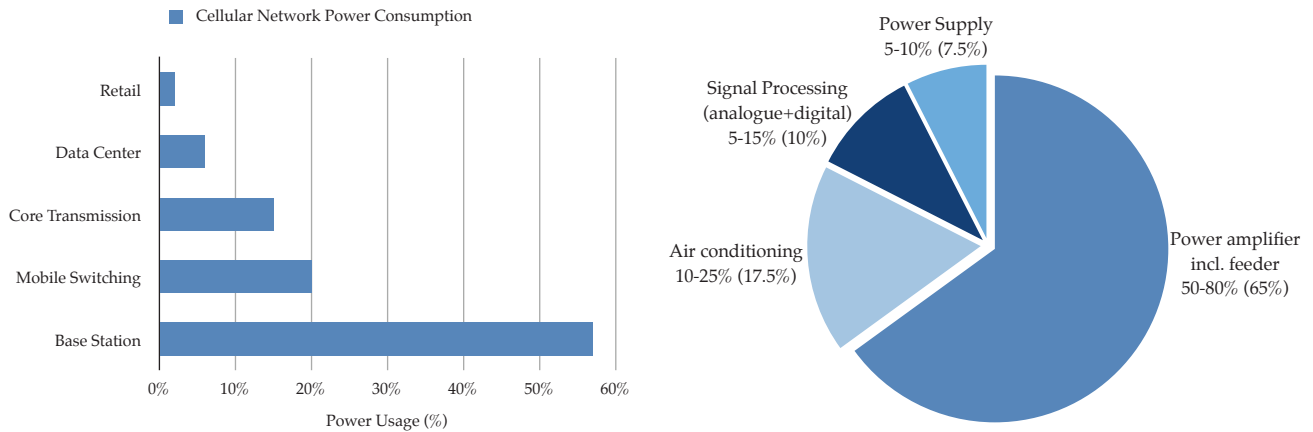
(a) Power consumption of a typical wireless cellular network [2](ref. therein) (b) Power consumption distribution in radio base stations [3](ref. therein)
