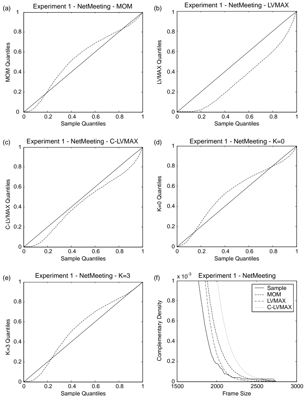
Fig. 4. Frame size histograms-Gamma models, Q-Q plots and complementary probability functions for terminal NM (experiment 1).
