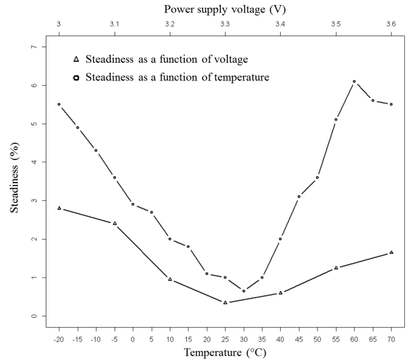
Fig. 12. Steadiness of responses generated using the MSB subtractor bit in a -20 °C to 70 °C temperature range (reference response at 25 °C) and in a 3.0 V to 3.6 V power supply voltage range (reference response at 3.3 V)
