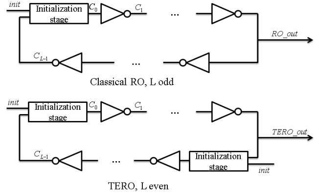
Fig. 1. Generic architecture of ROs and TEROs
