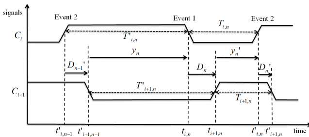
Fig. 6. Typical output chronogram of two adjacent TERO stages
