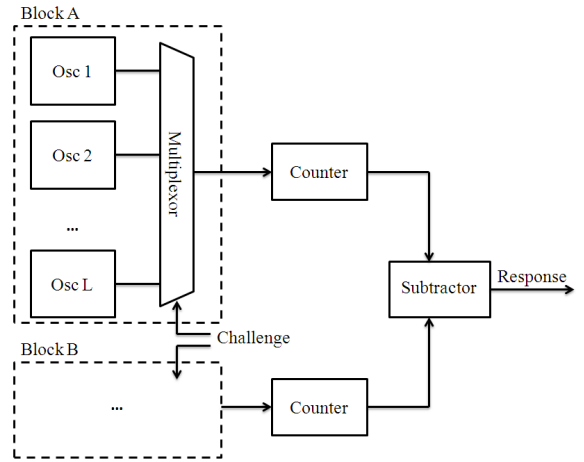
Fig. 3. Generic core architecture of RO-PUFs and TERO-PUFs
