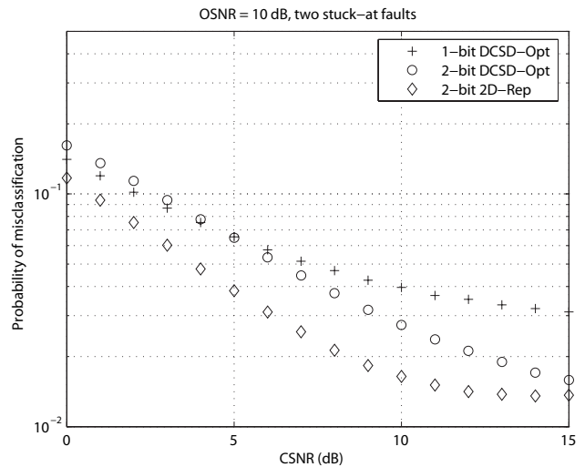
Fig. 4. Performance comparison of 1-bit DCSD-Opt, 2-bit DCSD-Opt, and 2-bit 2D-Rep at OSNR = 10 dB when two stuck-at faults are present.
