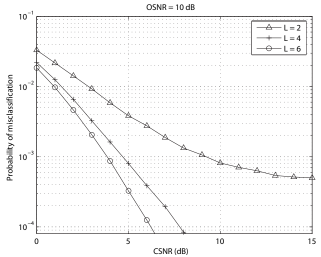
Fig. 3. Performance comparison of 2-bit, 4-bit, and 6-bit 2D-Rep at OSNR = 10 dB.
