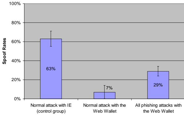
Figure 9. Spoof rates with and without the Web Wallet protection (including the standard errors)
