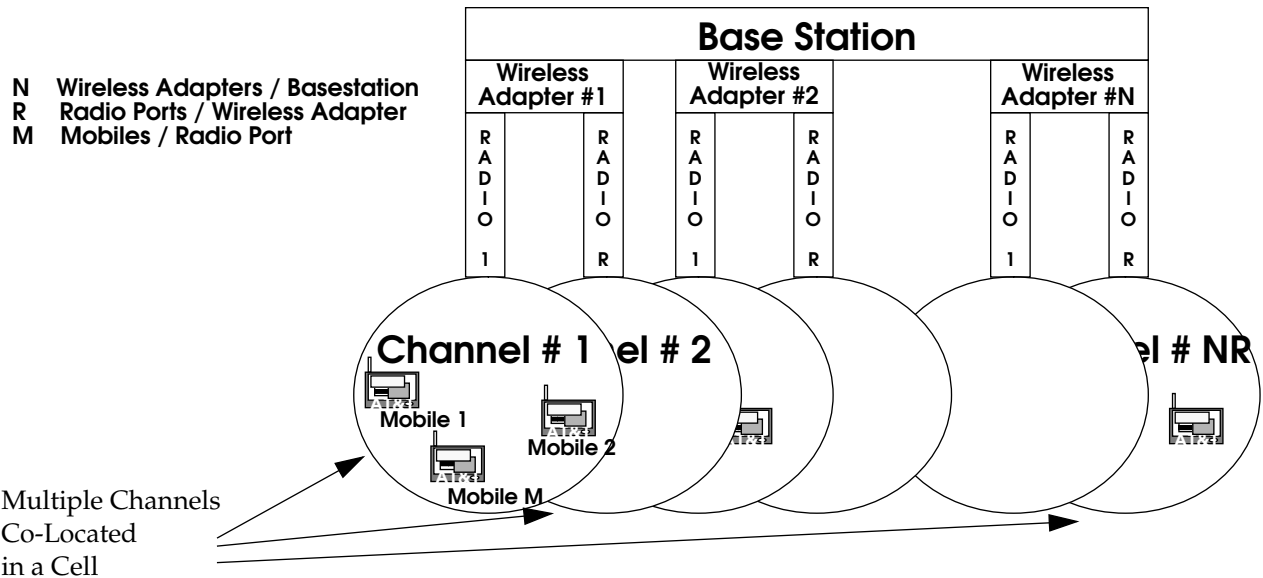
Figure 8: Abstract View of a Basestation in SWAN
