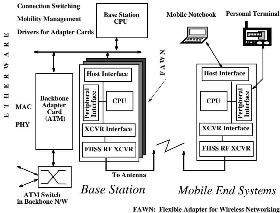
Figure 5: Architecture of SWAN System
