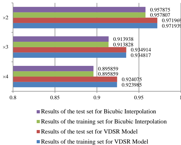
Fig. 13. SSIM Performance Comparison between the Training and Testing Results of VDSR Model and Bicubic Interpolation.
