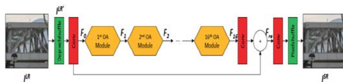
Fig. 3. The Architecture of Orientation-aware Deep Neural Network [13].
