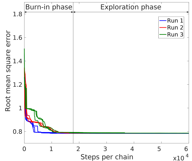
Figure 4. RMSE weighted by the standard deviation of the data error for the three inversion runs of the observed VSP data shown in Fig. 3. As the estimate of the standard deviation of the data error is fixed at a high value, the RMSE drops below 1. The vertical black line indicates the separation of the burn-in and the exploration phases, associated with the MCMC search of the parameter space.
