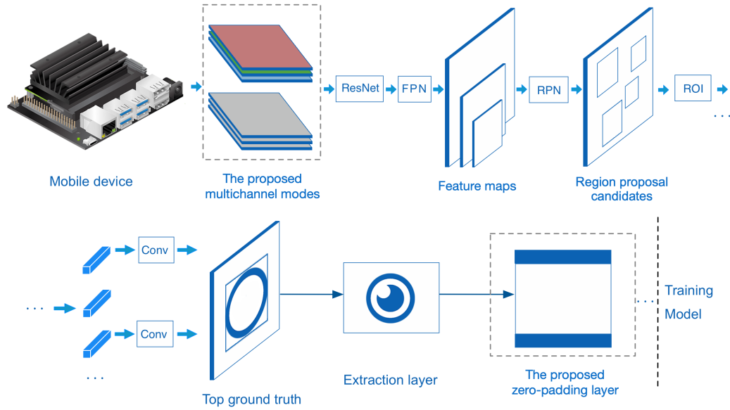
Fig 7. The optimized Mask R-CNN architectures in the mobile environment. The first dotted box illustrates that we implement two input modes are applied during the preprocessing of the system, VW(Color) and NIR(Grey) modes. The second dotted box illustrates that the non-holistic iris features map with discriminative information was obtained by Mask R-CNN and those scale-variant images are normalized by the custom zero-padding layers . Each individual component proposed in our Mask R-CNN architecture does influence iris recognition performance.
