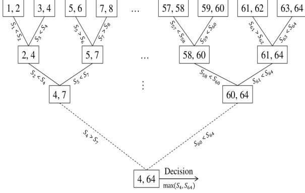
Figure 4: Tree structure based pairwise coupling.
