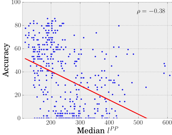
Figure 3: Accuracy versus median keypress latency showing the best-fit linear regression line
