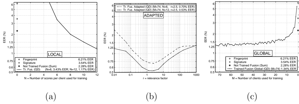
Fig. 1. Equal error rates of local (a), adapted (b), and global (c) approaches for multimodal fusion based on QDs.
