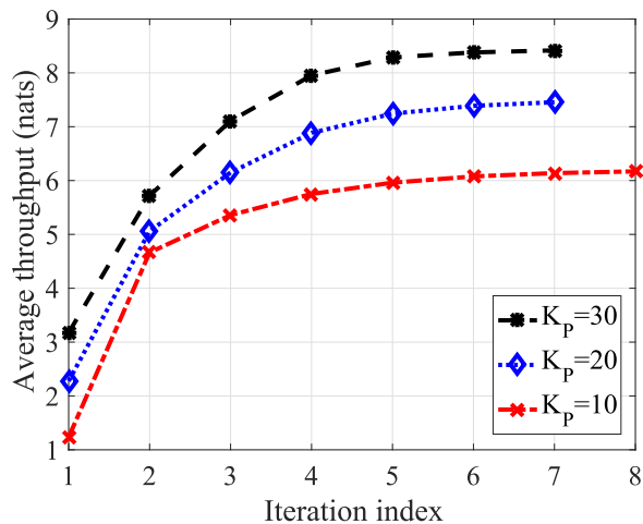
FIGURE 4. The convergence of Algorithm 1 for solving Problem I-C (MaxPRI) at M = 4, K_m = 20, P_m = 35 dBm.
