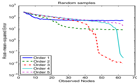
(a) Figure 1: Randomly-drawn Samples
