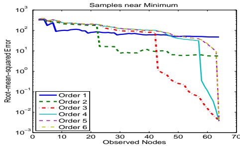
(c) Figure 3: Samples drawn near minimum
