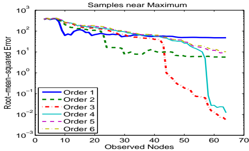
(b) Figure 2: Samples drawn near maximum
