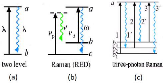
Figure 4. Various kinds of marker molecules. In every case \lambda is the wavelength of the incident light, \sin \theta = 0.83 and the refractive indices are n_1=1.9 while n_2=n_3=2.1 . (a) Two level scheme yields classical, one photon resolution. (b) Raman eraser doublet (RED) scheme as discussed in the text. (c) Three photon Raman scheme that requires correlation between three detectors.
