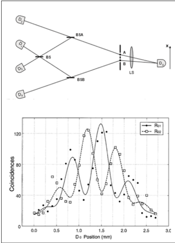
Figure 2. (Top) Proposed quantum eraser experiment. A pair of entangled photons is emitted from either atom A or atom B by atomic cascade decay. “Clicks” at D_3 or D_4 provide the which-path information and clicks at D_1 or D_2 erase the which-path information. (Bottom) R_{01} and R_{02} against the x coordinates of detector D_0 . Standard Young’s double-split interference patterns are observed. Note the \pi phase shift between R_{01} and R_{02} . The solid line and dashed line are fits to the data based on Eq.(6) in Ref.[5].
