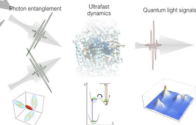
Fig. 1 An entangled photon pair probes the ultrafast dynamics in a molecular system via the pump-probe technique. Due to the unique temporal and spectral parameters of entangled light, the spectroscopic signal obtained by quantum light carries molecular information not accessible by classical light.
