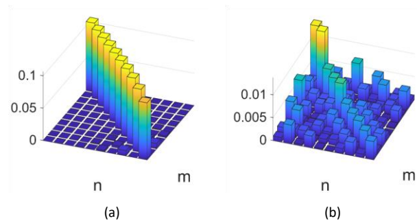
Figure 2. The reduced density-matrix of the idler beam in the Schmidt basis using Hermite-Gaussian modes. (a) The idler's reduced density matrix in Eq. (1) before the interaction with the object presented in Hermite-Gauss basis modes. (b) The change in the reduced density matrix of the idler due to the interaction with the object in Eq. (2). The induced coherence (o -diagonal elements) reveal matter information transfer from the signal to the idler.
