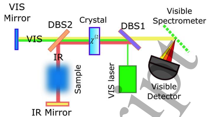
Figure 1 – The scheme of the nonlinear Michelson interferometer used for ISVL. Visible and IR photons are generated in a crystal pumped the laser. The visible and IR photons are split on the dichroic beamsplitter (DBS) and then reflected into the crystal by respective mirrors. The sample is inserted in the path of IR photons. The interference pattern for visible photons is detected using the visible range spectrometer and the detector. The pattern depends on properties of the sample, which interacts with the IR photon.
