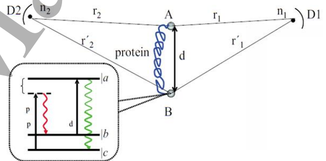
Figure 3. Marker molecules or quantum dots at A and B generate correlated pairs of photons by a Raman quantum eraser process in which the scatterers are pumped by a laser (frequency \nu_p ) to a virtual level (dashed line) and spontaneously emit the first (Stokes) photon ( \nu ). The molecule is then promoted from b \rightarrow a by absorbing a drive laser photon (frequency \nu_d ) and spontaneously emits the second (anti-Stokes) photon ( \omega ). The medium on the right (left) half plane has refractive index n_1=1.9 ( n_2=2.1 ).
