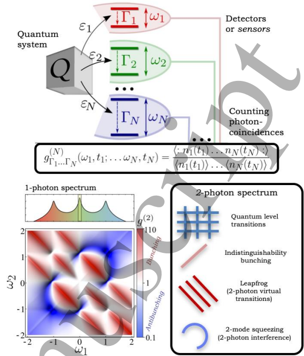
Figure 1 — Scheme of the sensors method with an example of a 2-photon spectrum (2PS) with signature features.
