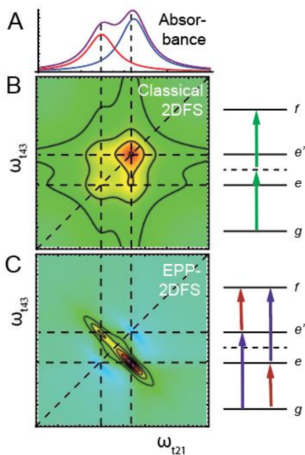
Figure 1. Simulated absorbance (A), classical 2DFS (B), and EPP-2DFS (C) for an electronically coupled molecular dimer. For both 2DFS and EPP-2DFS, transition energy level diagrams are shown on the right. The temporal-spectral correlation of the EPP state effectively “windows” the classical 2DFS spectrum, facilitating the detection of cross-peak features. Adapted from ref. [2].
