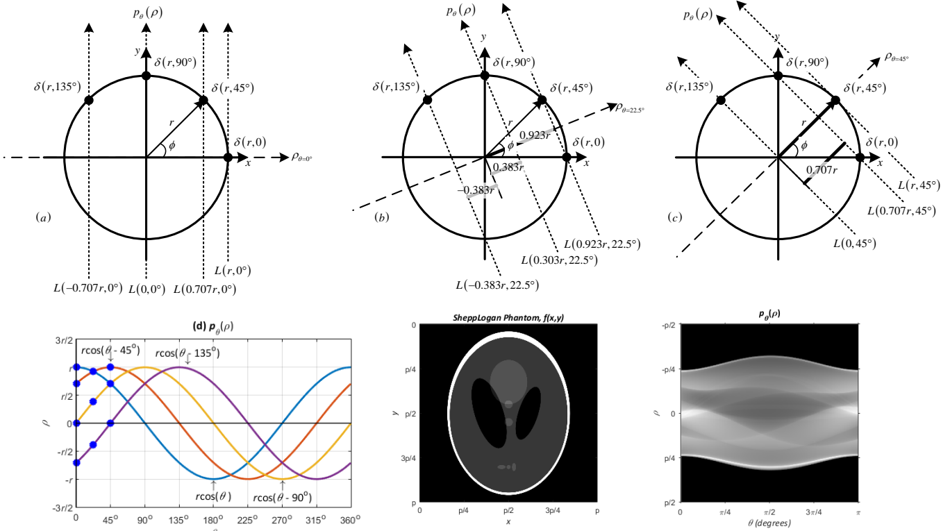
Fig. 5. Rotating L(\theta, \rho) to scan \delta(r, \phi) and Line mass “point spread function” for \phi = 0, 45^\circ, 90^\circ, 135^\circ and the Sinogram of Shepp-Logan head phantom
