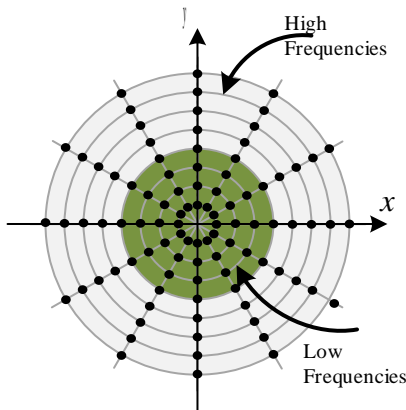
Fourier Sampling with Fourier Slice Theorem
