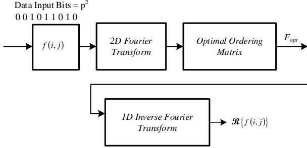
Fig. 9. Data Symbols Generation using FRAT
