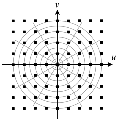
Sampling Required by Fast Fourier Transform
