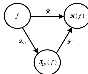
Fig. 1. The Relation between Radon Transform and Fourier Transform
