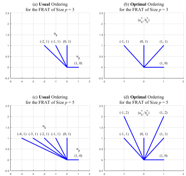
Fig. 8. The Set of Normal Vectors, which Indicate the Represented Directions for p = 3 & 5
