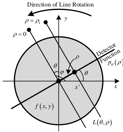
Fig. 2. Radon Transform Demonstration
