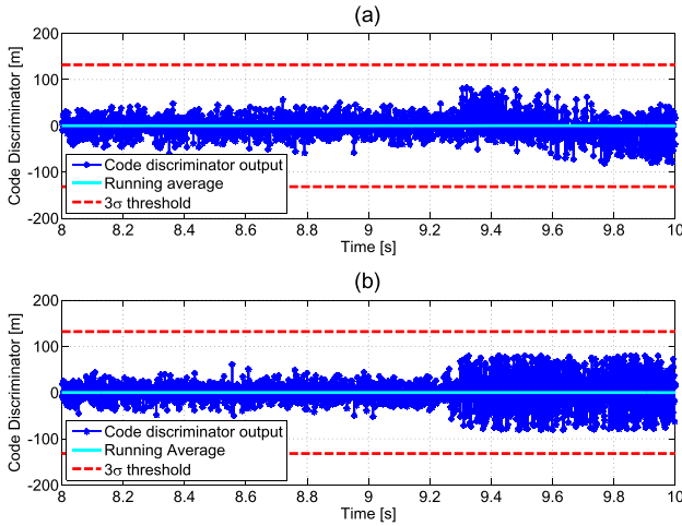
Fig. 6. GPS L1 C/A tracking performance: code discriminator output in the presence of a -130\text{-dBW} in-band CWI (top) and in the presence of a single-saw-tooth chirp signal at -130\text{ dBW} (bottom).
