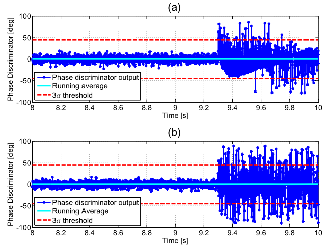
Fig. 7. GPS L1 C/A tracking performance: carrier discriminator output in the presence of a -130\text{-dBW} in-band CWI (top) and in the presence of a single-saw-tooth chirp signal at -130\text{ dBW} (bottom).
