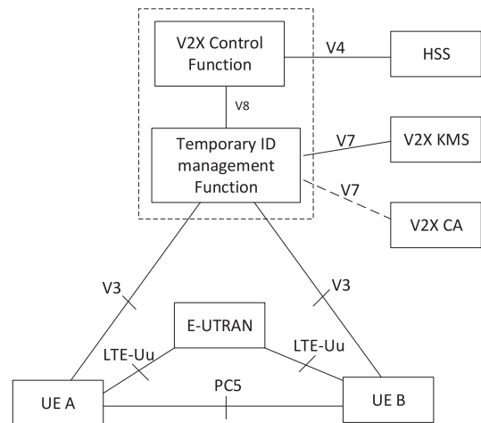
FIGURE 8. Security architecture for V2X communications (PC5 and LTE-Uu based) [91].
