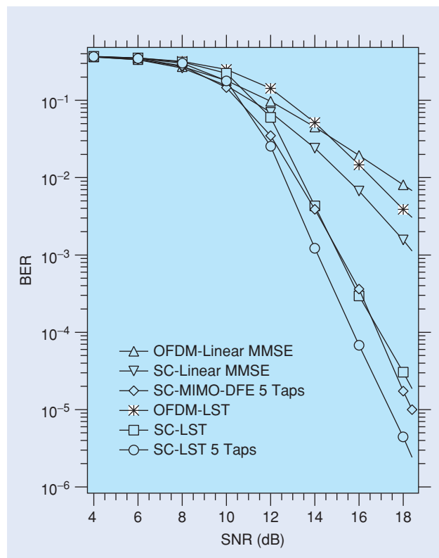
[FIG15] BER performance of various OFDM and SC receivers operating over a 4 \times 4 six-ray channel. Convolutional coding with 64 states rate 3/4 is used.
