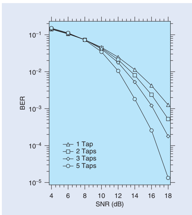
[FIG9] BER for different feedback taps for MIMO-DFE.
