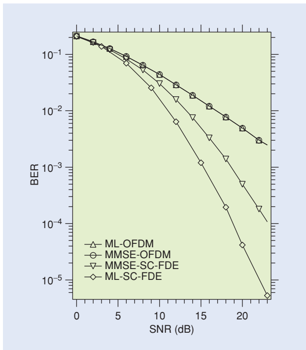
[FIG10] Performance comparison of two SC systems employing FDE with two OFDM systems. Ideal CSI at the receive side and SISO scenario are assumed.
