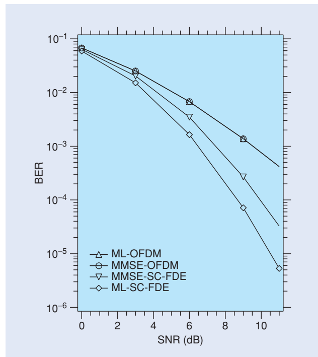
[FIG11] Performance comparison of two SC systems employing FDE with two OFDM systems. Ideal CSI at the receive side and SIMO scenario with three receive antennas are assumed.
