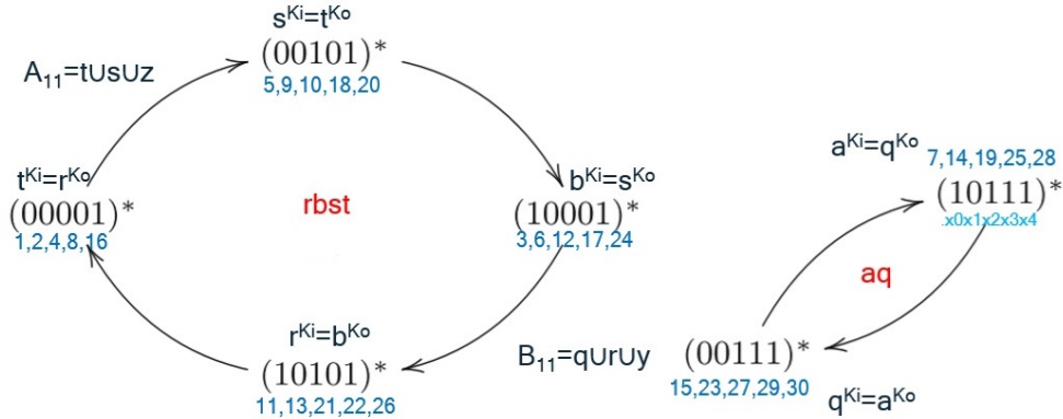
Fig. 2. Canonical states with Keccak S-box cf. [ScDa24] vs. notations of this paper.
